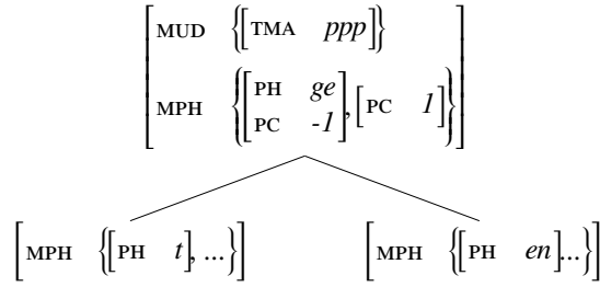
Figure 6: Vertical abstraction by inheritance
